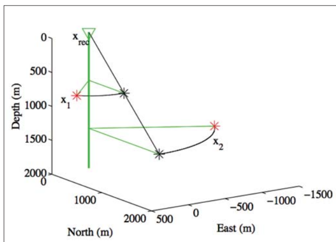
Figure 3. The receiver in a 1D array is (vertically) stationary with respect to two given sources (red stars) if the source locations can be rotated about the receiver line into collinear positions (black stars).
